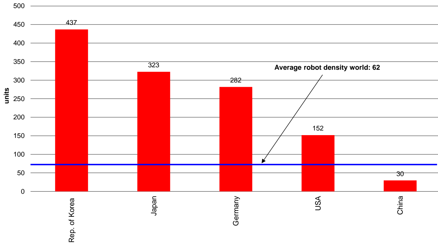
Robot density in the five biggest destinations of robot supplies in 2014
